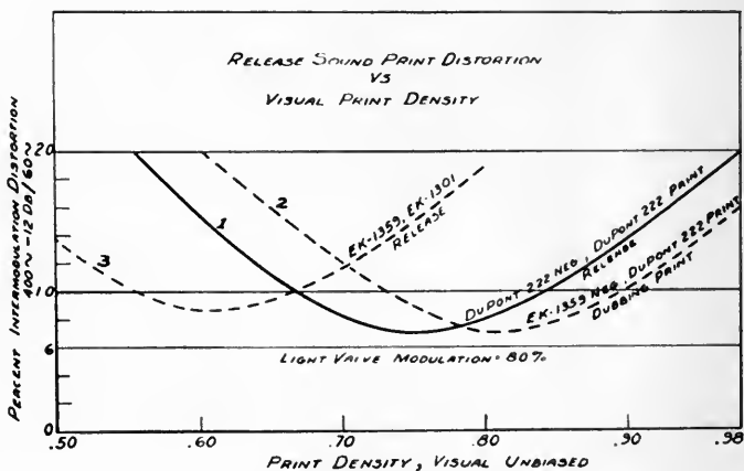
FIG. 8. Intermodulation distortion curves for (a) fine-grain release prints; (b) fine-grain dubbing prints; and (c) normal positive stock release prints.
